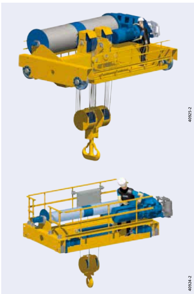
32-tonne MPW crab with special switchgear cabinet fitting
